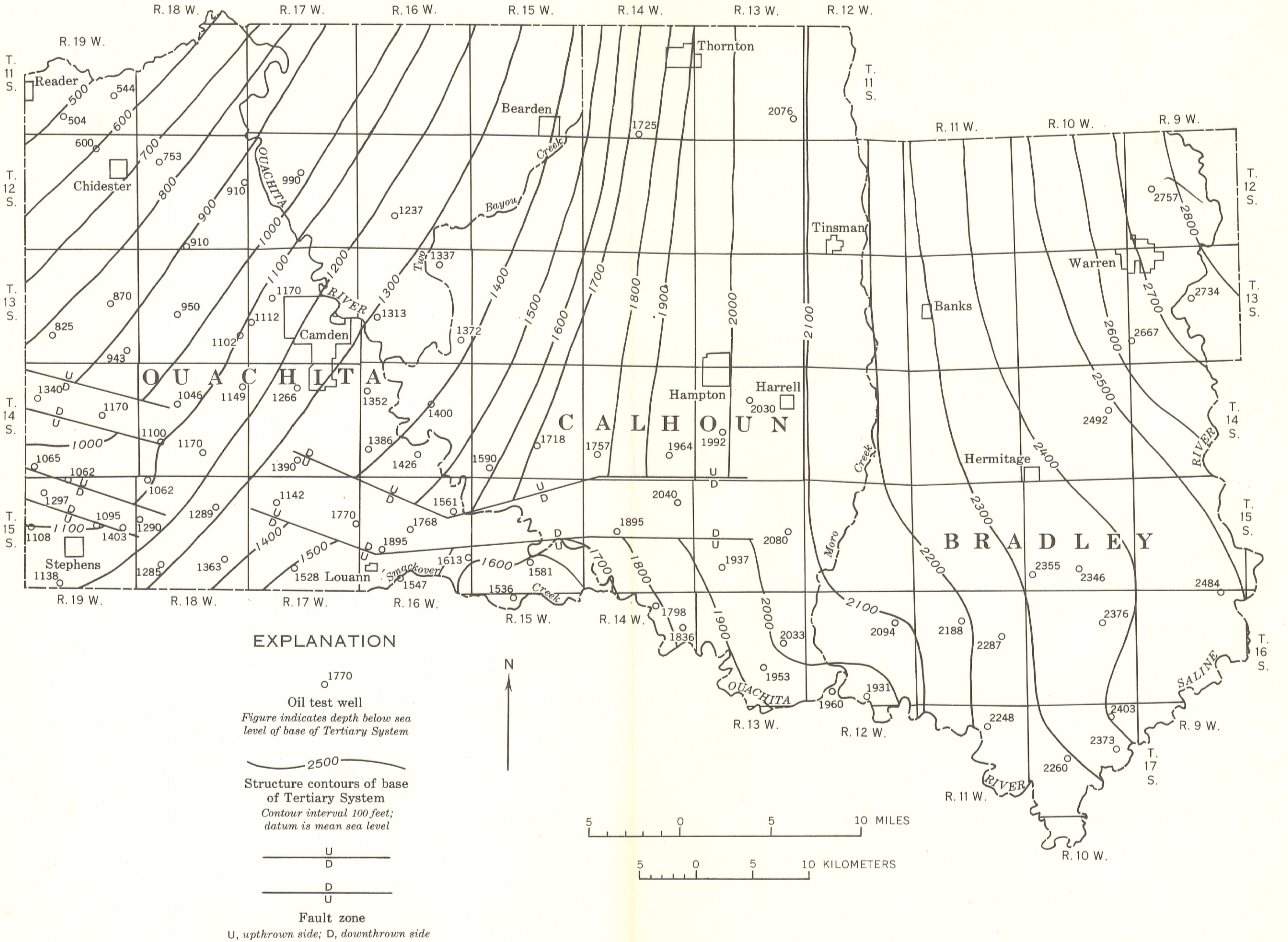
STRUCTURE CONTOUR MAP OF BRADLEY, CALHOUN, AND OUACHITA COUNTIES, ARKANSAS
