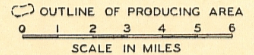
STRUCTURE CONTOUR MAP OF UNION COUNTY ARKANSAS - CONTOURS DRAWN ON TOP OF MEAKIN SAND (TOP OF OZAN FORMATION) CONTOUR INTERVAL 25 FEET - FIGURES GIVE DEPTHS BELOW SEA LEVEL
