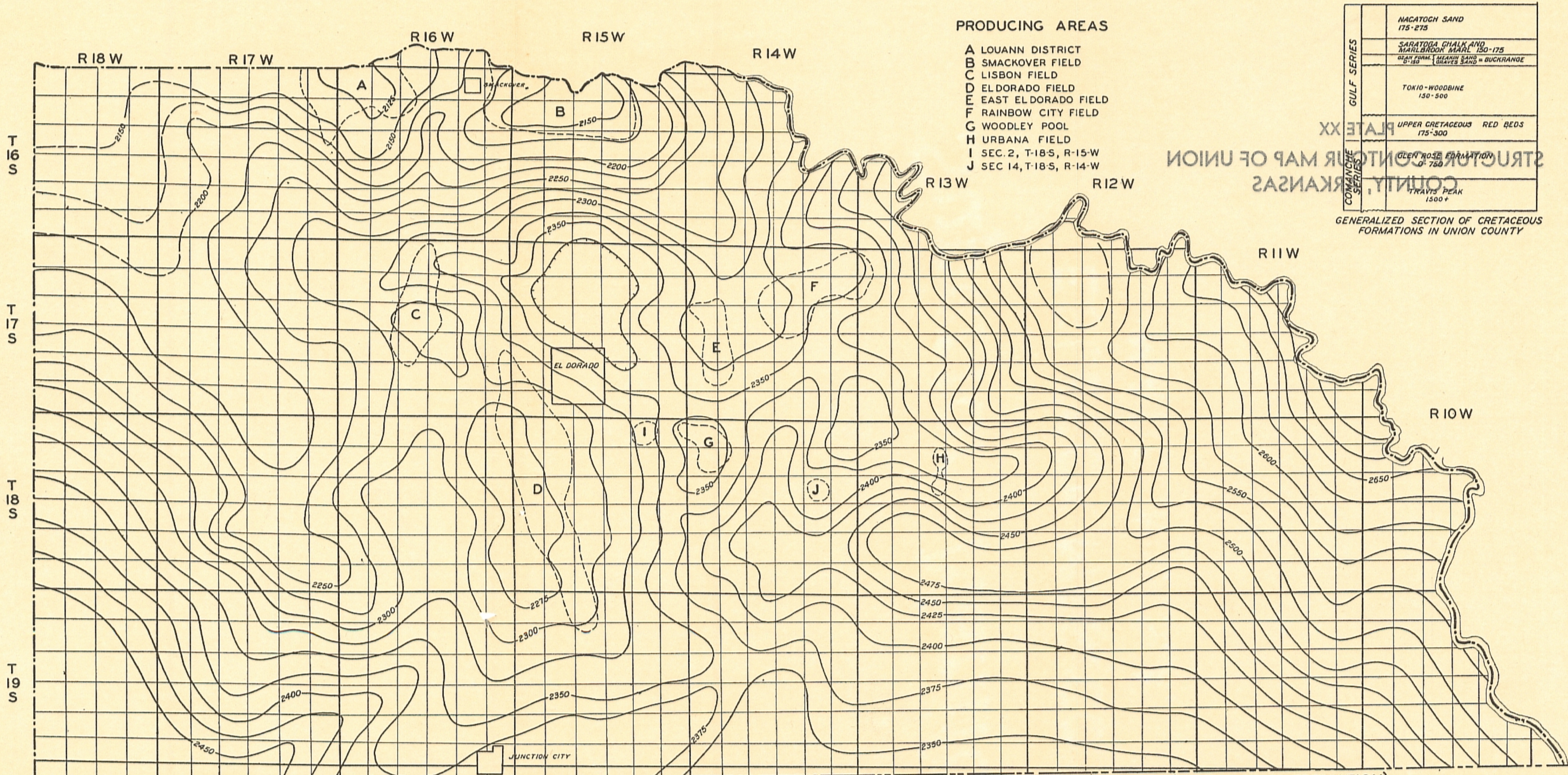
STRUCTURE CONTOUR MAP OF UNION COUNTY ARKANSAS - CONTOURS DRAWN ON TOP OF MEAKIN SAND (TOP OF OZAN FORMATION) CONTOUR INTERVAL 25 FEET - FIGURES GIVE DEPTHS BELOW SEA LEVEL
