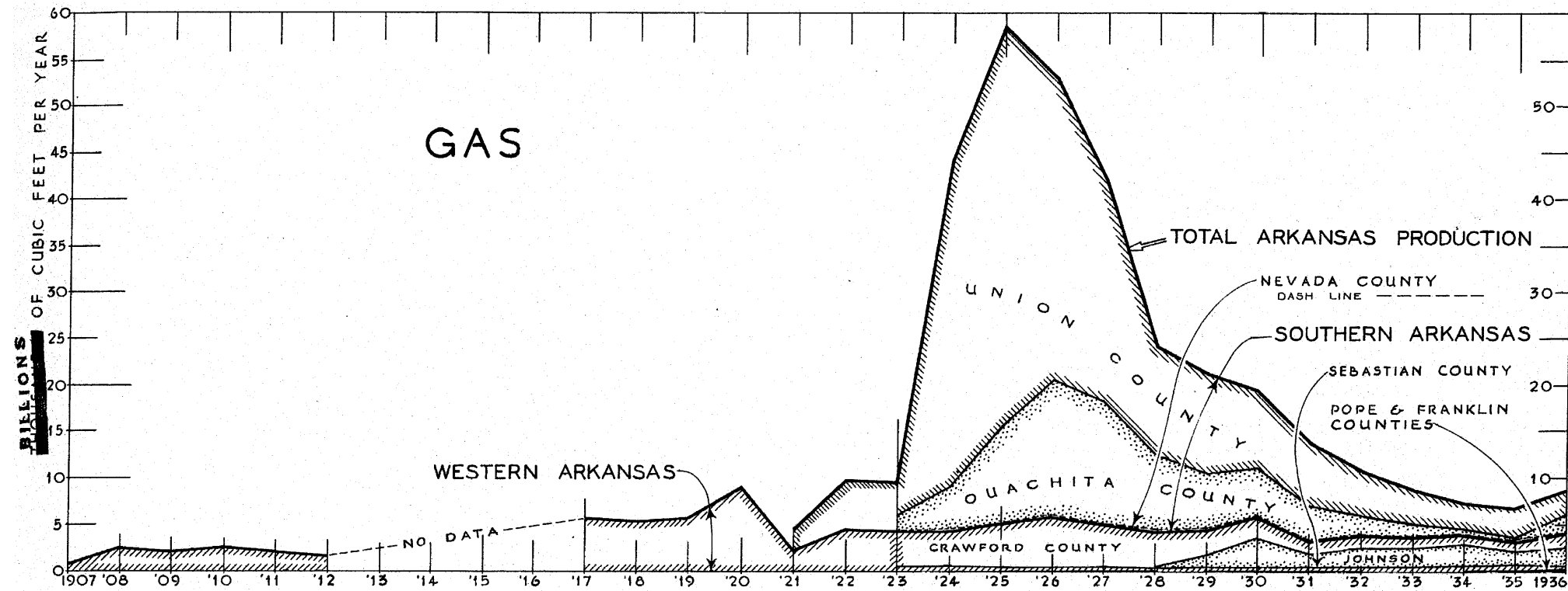
FIG. 1A, GRAPH SHOWING ARKANSAS NATURAL GAS PRODUCTION, 1907-1936. SOURCE: U.S. GEOLOGICAL SURVEY, U.S. BUREAU OF MINES, AND SEVERANCE TAX REPORTS FILED WITH STATE DEPARTMENT OF REVENUES.
