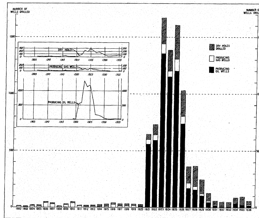
FIGURE 6. CHART SHOWING NUMBER OF OIL WELLS, GAS WELLS, AND DRY HOLES DRILLED IN ARKANSAS FROM 1902 TO 1936, INCLUSIVE SOURCE OF INFORMATION: "PETROLEUM IN THE UNITED STATES AND ITS POSSESSIONS," BY WILLIAM J. KEMMERTZ AND RALPH ARNOLD, 1931, U.S. GEOLOGICAL SURVEY, U.S. BUREAU OF MINES, AND ARKANSAS BOARD OF CONSERVATION.
