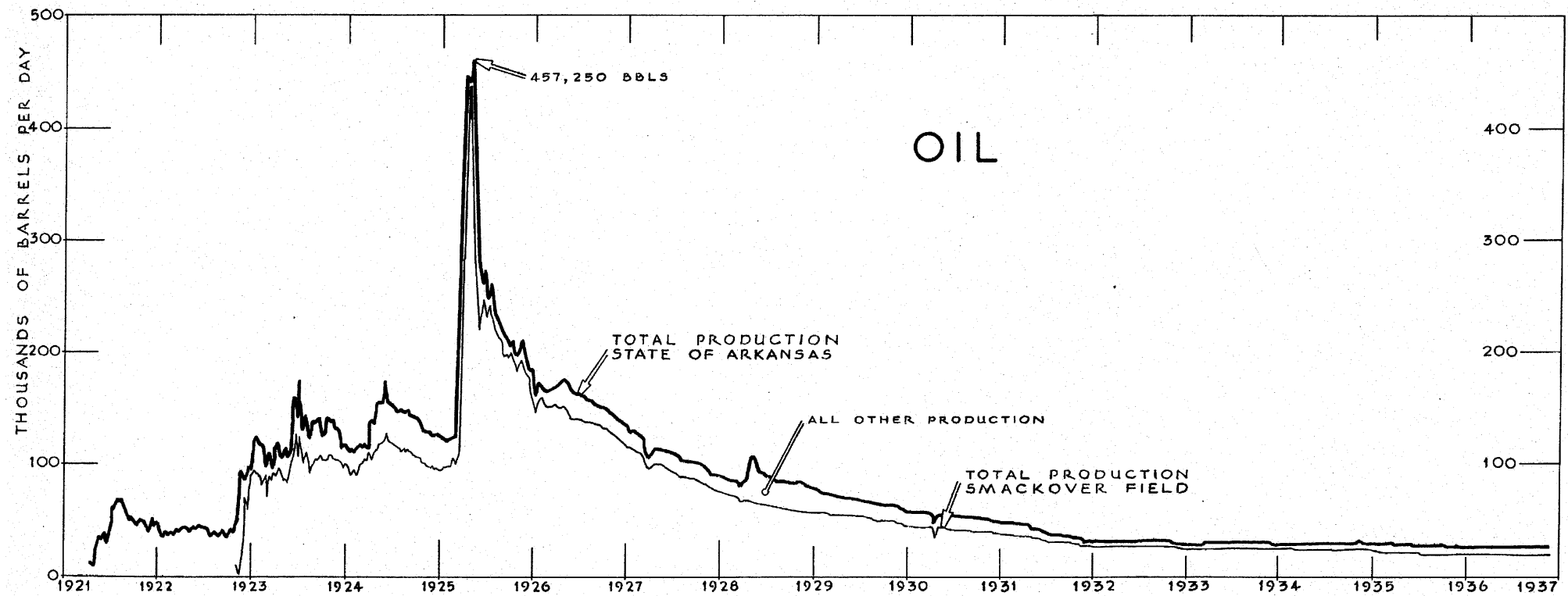
FIG. 1B, GRAPH SHOWING DAILY AVERAGE PETROLEUM PRODUCTION STATE OF ARKANSAS AND SMACKOVER FIELD, 1921-1936. SOURCE: AMERICAN PETROLEUM INSTITUTE.
