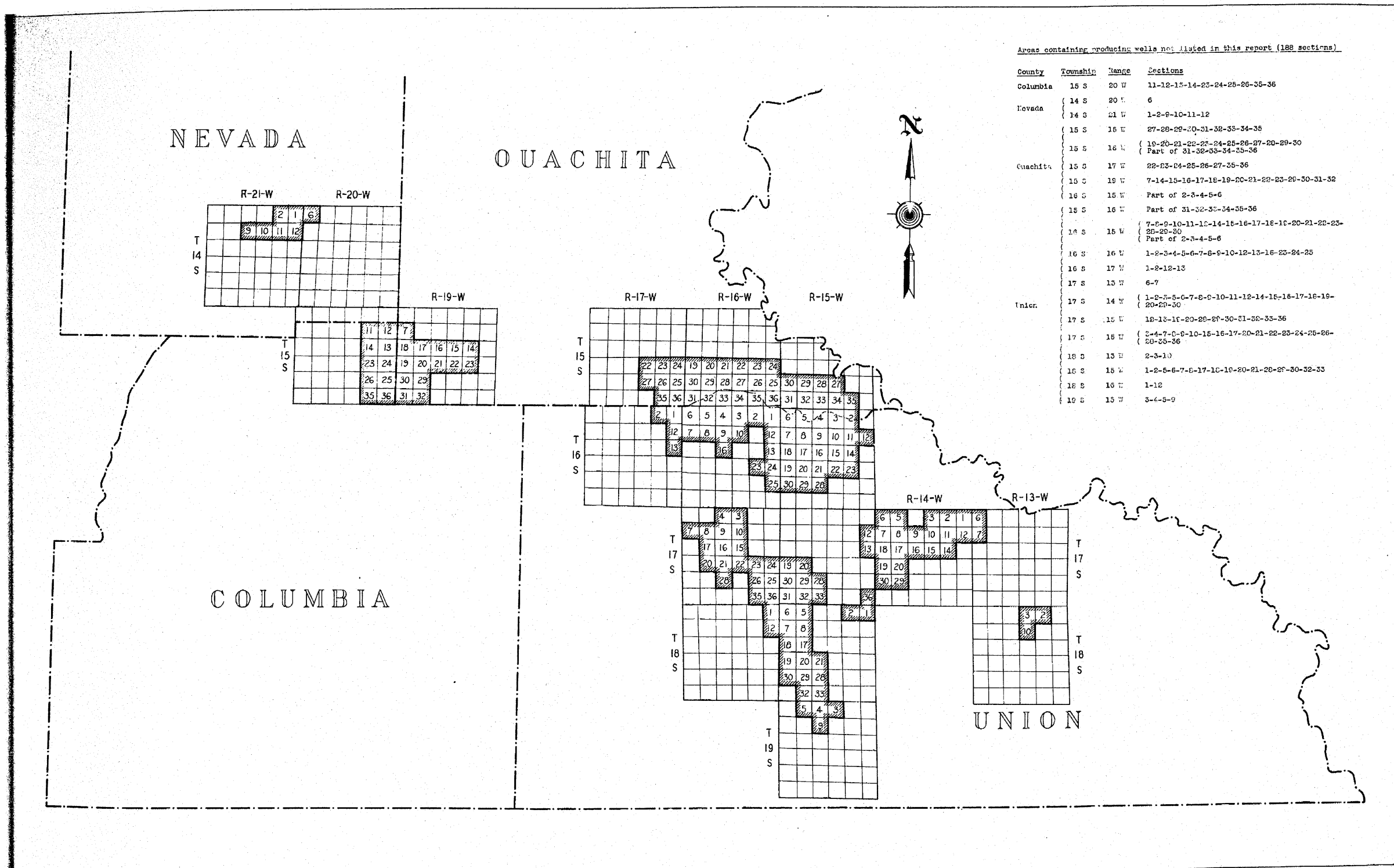
FIGURE 5. INDEX MAP SHOWING AREAS CONTAINING PRODUCING WELLS NOT LISTED IN THIS REPORT (188 SECTIONS)
