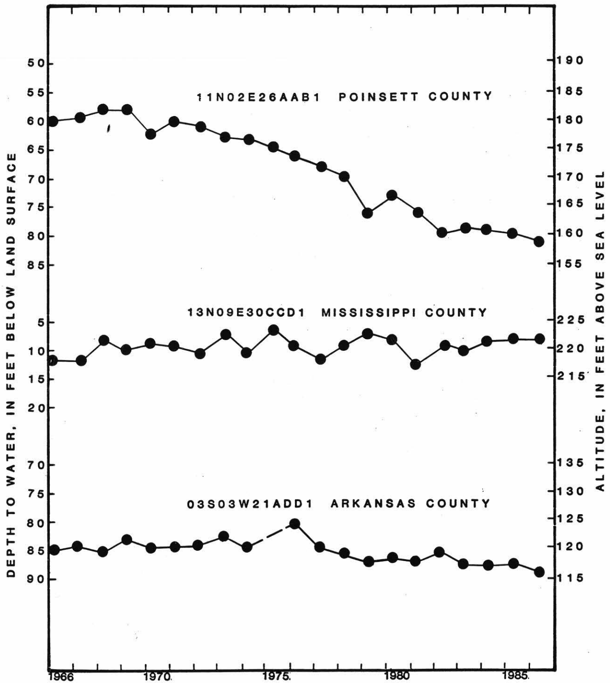
Figure 1. Sheet 1 of 2.--Water-level hydrographs for selected wells completed in Quaternary deposits.
