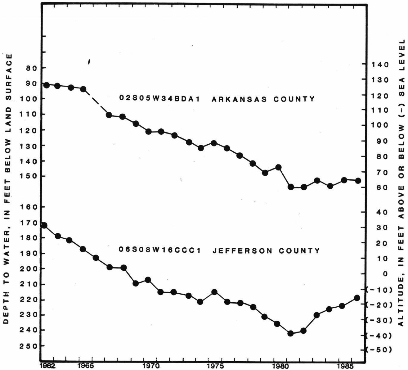
Figure 2. sheet 1 of 2.--Water-level hydrographs for selected wells completed in the Sparta Sand.
